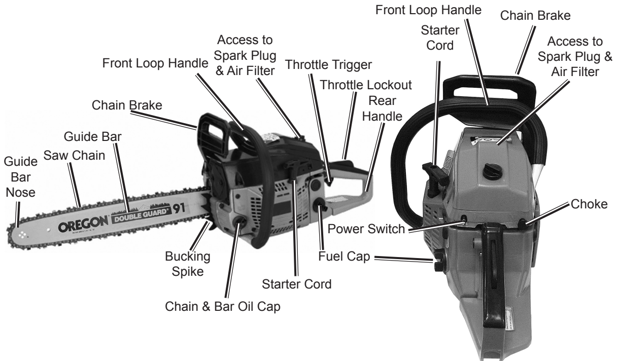
Figure 2 - Model 66909 18" 45cc Chain Saw
