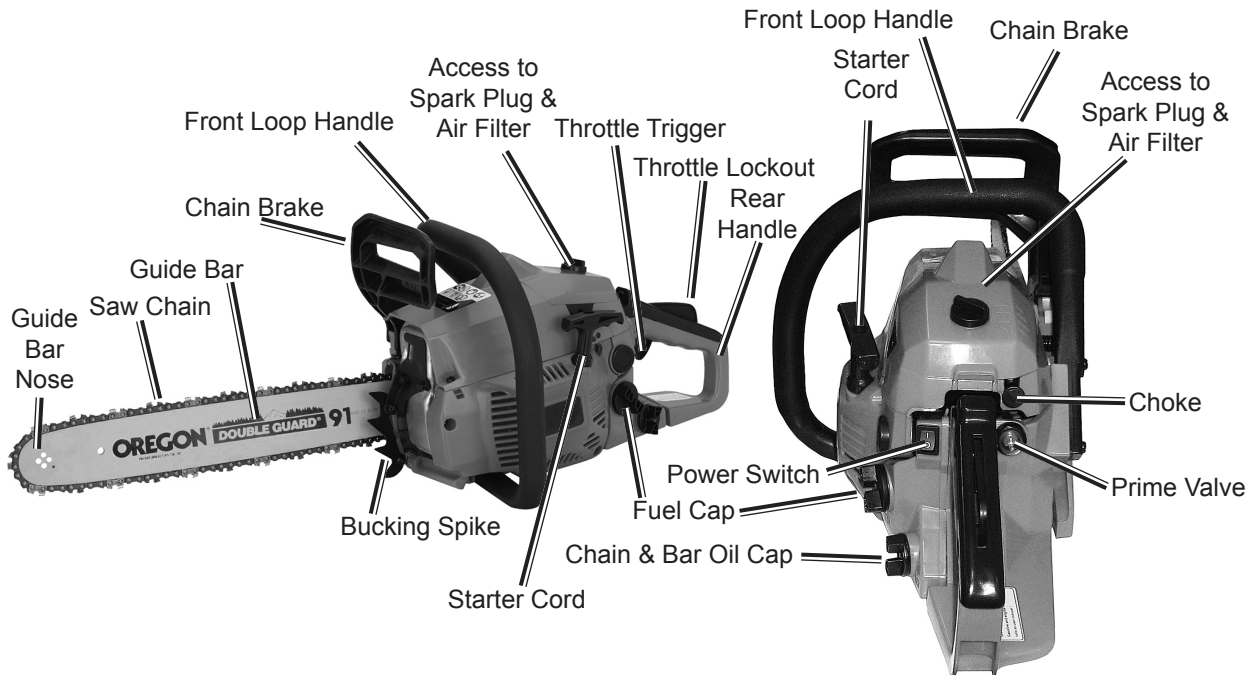
Figure 1 - Model 66908 16" 37cc Chain Saw
